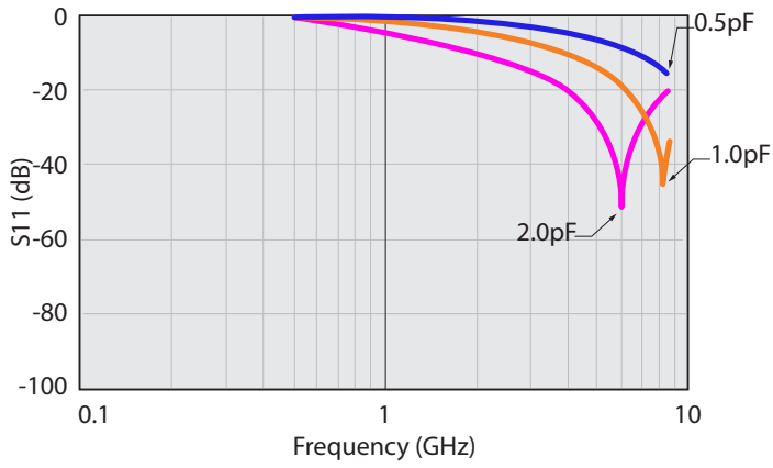
S11 vs. Frequency
