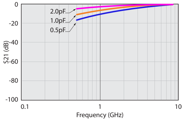
S21 vs. Frequency
