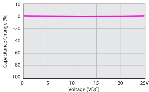
Capacitance - DC Voltage Characteristics
