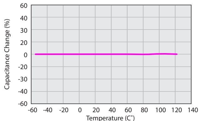
Capacitance - Temperature Characteristics
