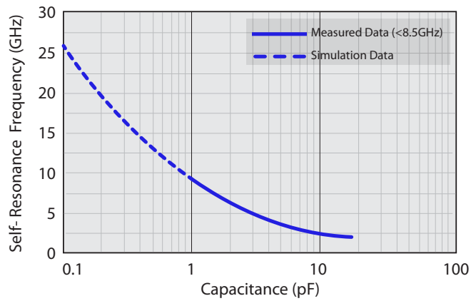
Self- Resonance Frequency vs. Capacitance
