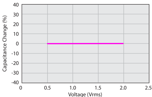
Capacitance - AC Voltage Characteristics
