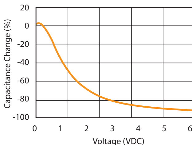
2. Capacitance vs. DC Voltage
