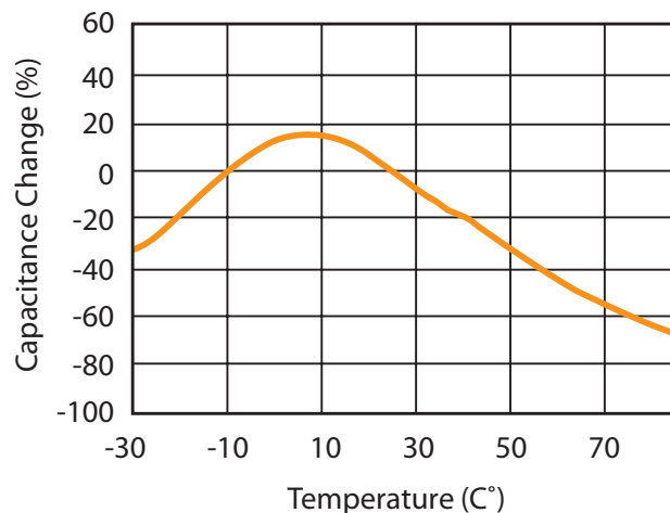
4. Capacitance vs. Temperature
