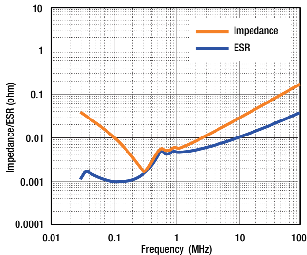
1. Impedance /ESR - Frequency
