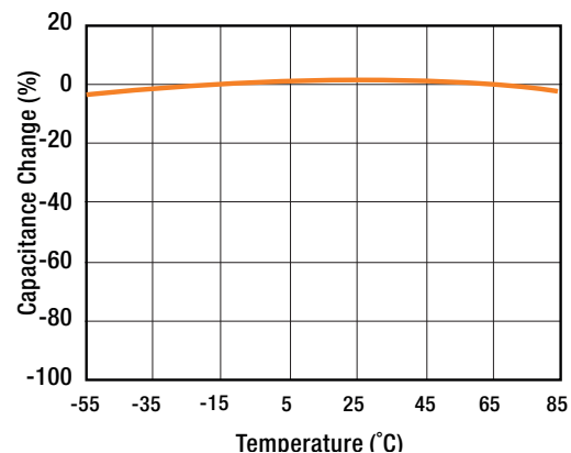
5. Capacitance - Temperature Characteristics
