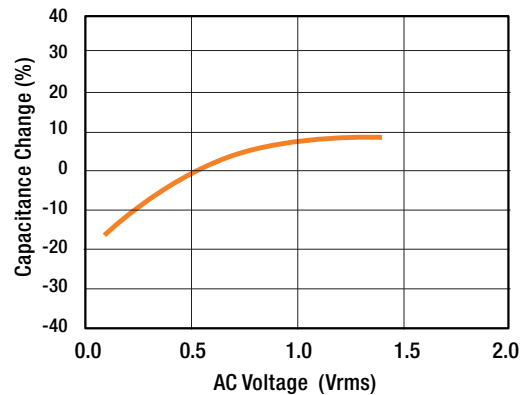
3. Capacitance - AC Voltage Characteristics
