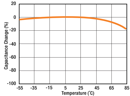
5. Capacitance - Temperature Characteristics
