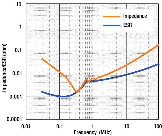
1. Impedance /ESR - Frequency
