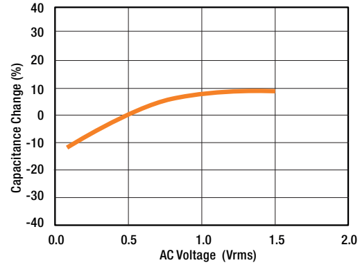
3. Capacitance - AC Voltage Characteristics
