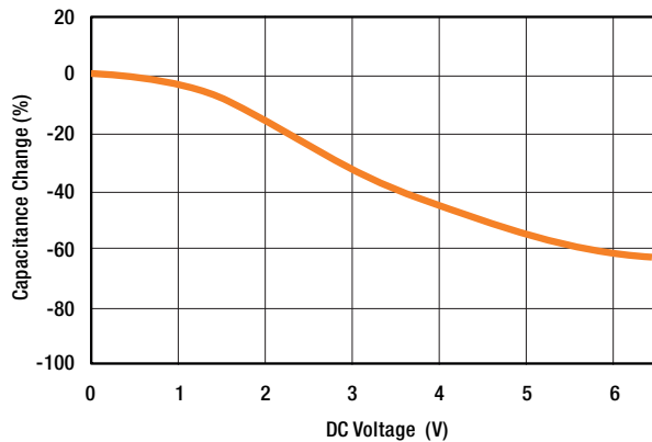
2. Capacitance - DC Voltage Characteristics
