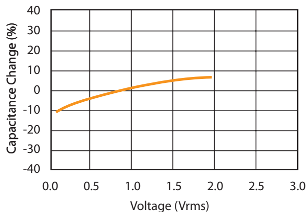
3. Capacitance vs. AC Voltage
