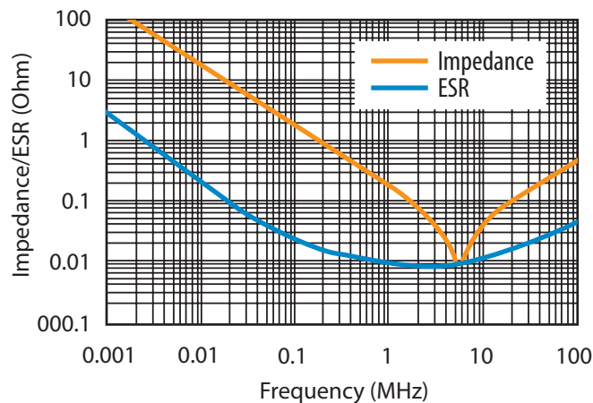
1. Impedance/ESR vs. Frequency
