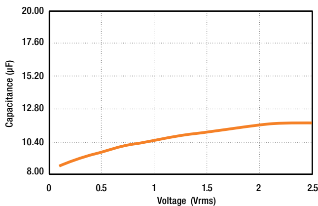
3. Capacitance vs. AC Voltage
