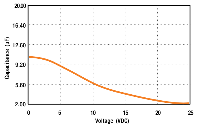
2. Capacitance vs. DC Voltage
