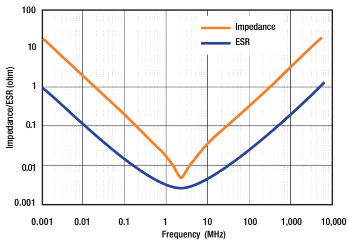
1. Impedance /ESR vs. Frequency
