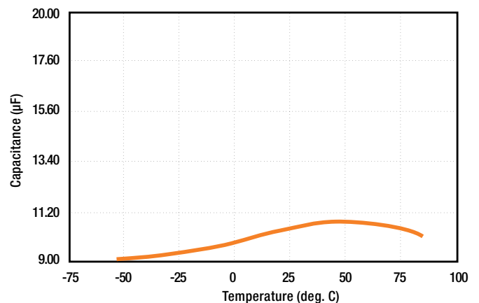
4. Capacitance vs. Temperature
