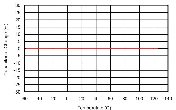
4. Capacitance-Temperature Characteristics
