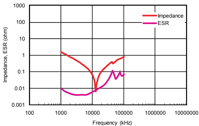
1. Impedance/ESR - Frequency
