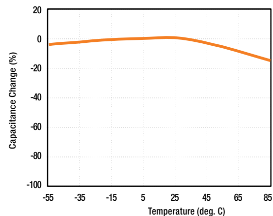
4. Capacitance vs. Temperature
