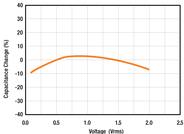
3. Capacitance vs. AC Voltage
