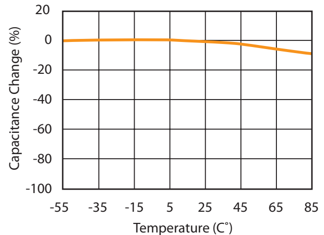
4. Capacitance vs. Temperature
