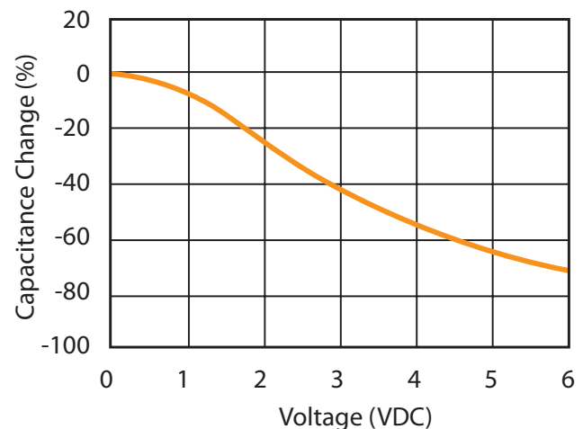
2. Capacitance vs. DC Voltage
