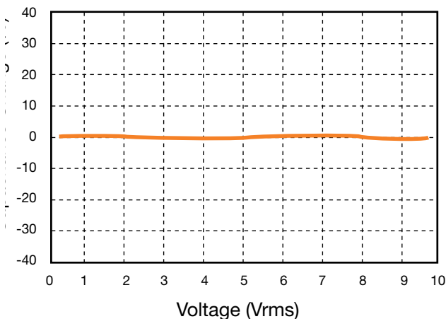
Capacitance vs. AC Voltage
