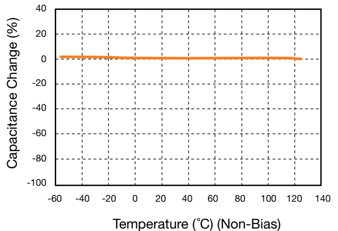
4. Capacitance vs. Temperature
