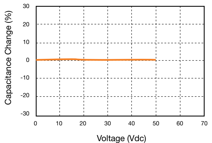
2. Capacitance vs. DC Voltage
