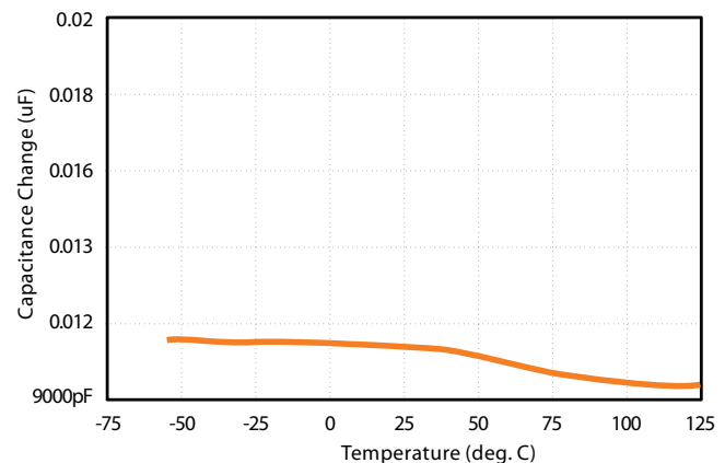
4. Capacitance vs. Temperature
