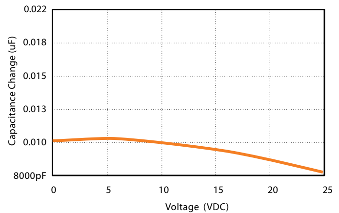
2. Capacitance vs. DC Voltage
