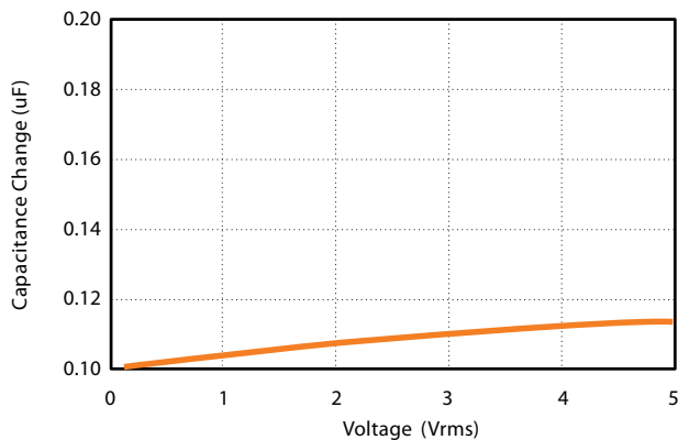
3. Capacitance vs. AC Voltage
