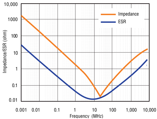
1. Impedance /ESR vs. Frequency
