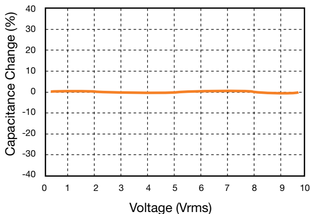
3. Capacitance vs. AC Voltage
