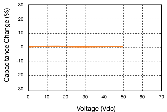
2. Capacitance vs. DC Voltage
