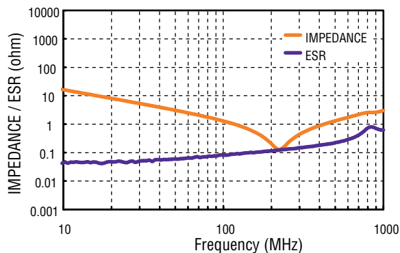
1. Impedance /ESR vs. Frequency
