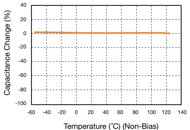
4. Capacitance vs. Temperature
