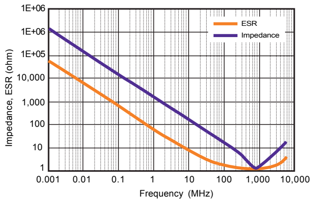
1. Impedance /ESR vs. Frequency
